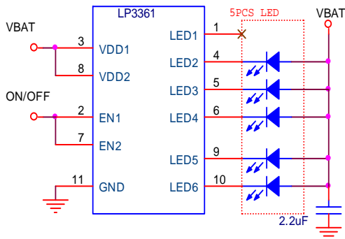
LP3361 Driver 5pcs White-LED Application
