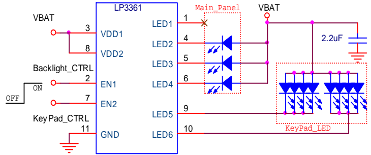
LP3361 Driver Panel and Keypad WLED Application
