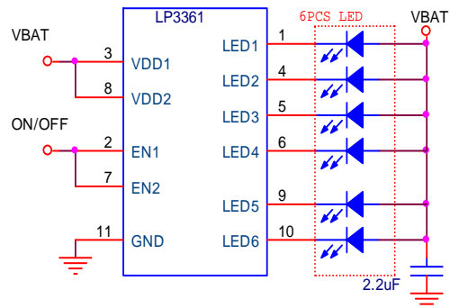
LP3361 Driver 6pcs White-LED Application
