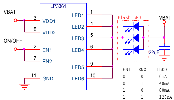
LP3361 Driver Flash White-LED Application
