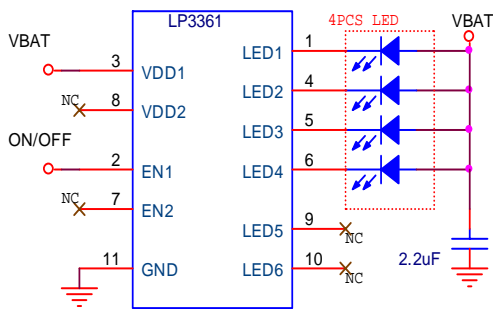
LP3361 Driver 4pcs White-LED Application
