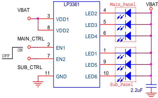
LP3361 Driver Dual Panel Application
