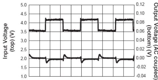
Time (100μs/div)
