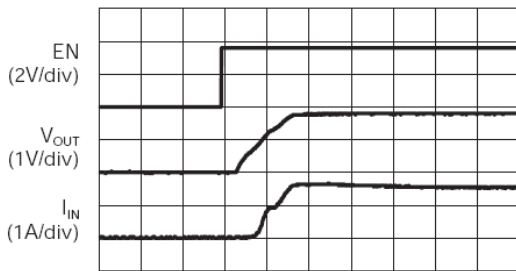
Time (100μs/div)
