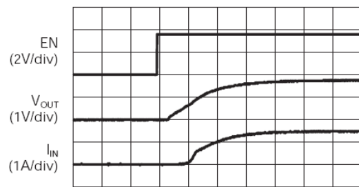
Time (100μs/div)
