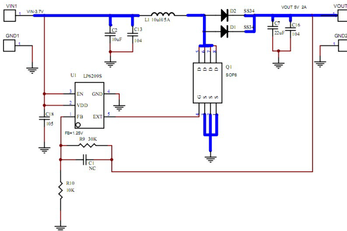
Figure3: Boost from 3.7V to 5V 3.1A
