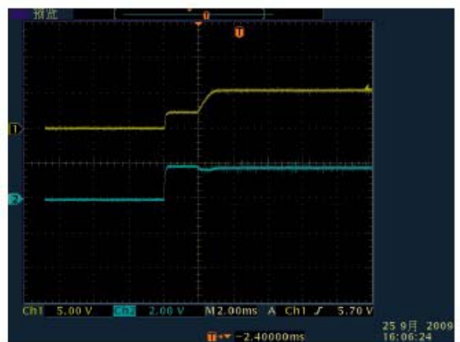
Iout=100mA
