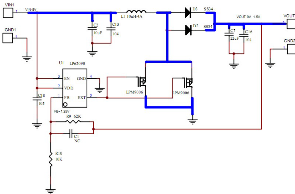
Figure4: Boost from 3.7V to 9V 1.5A
