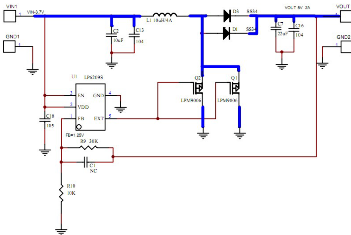
Figure2: Boost from 3.7V to 5V 2A
