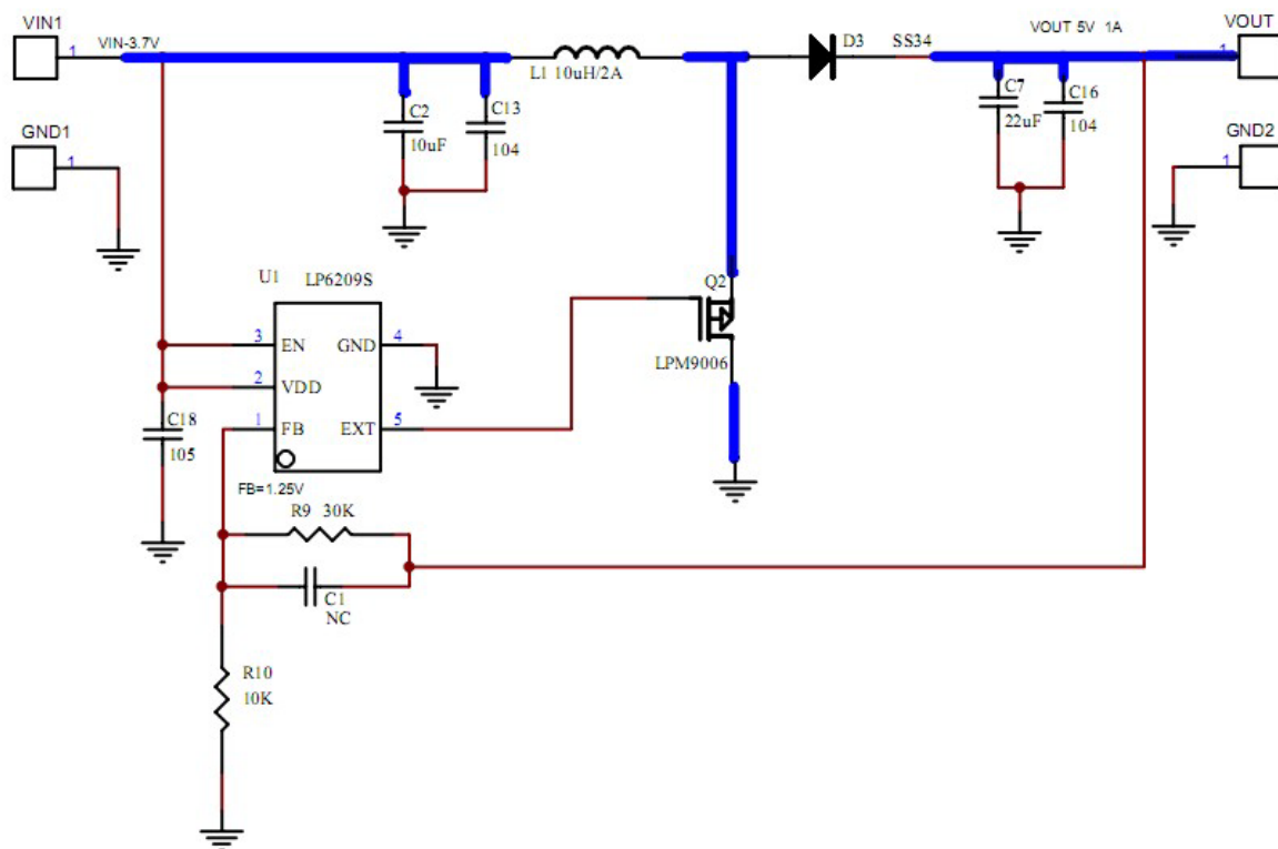
Figure1: Boost from 3.7V to 5V 1A
