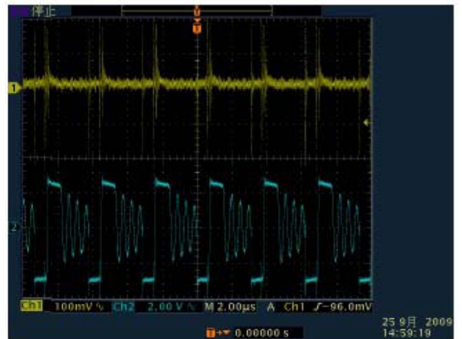
Iout=10mA
