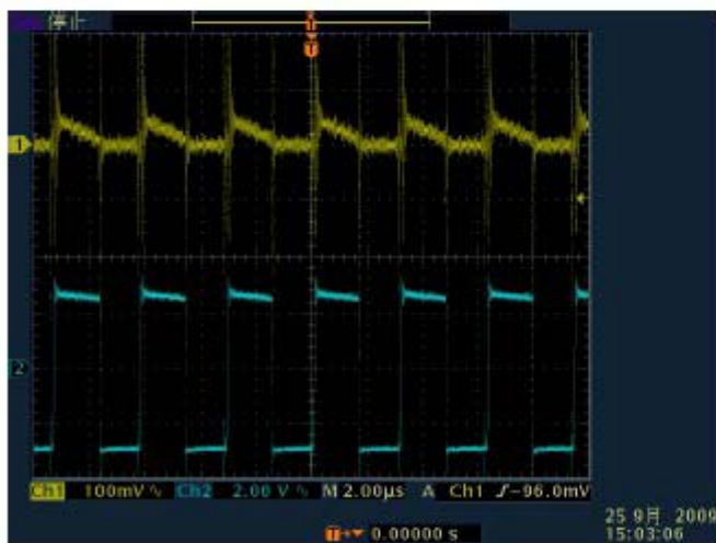
Iout=100mA
