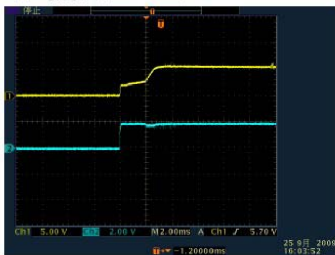
Iout=1mA
